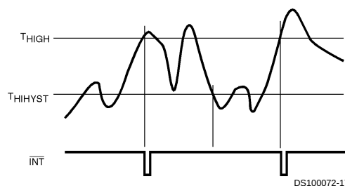
FIGURE 12. One-Time Interrupt Response Diagram
