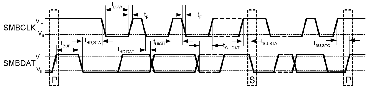
SMBus Communication
