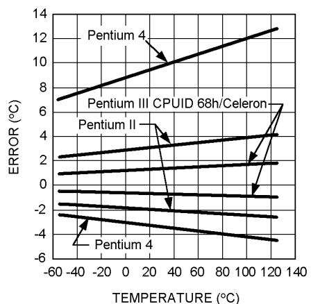
10130337 Error Caused by Non-Ideality Factor
