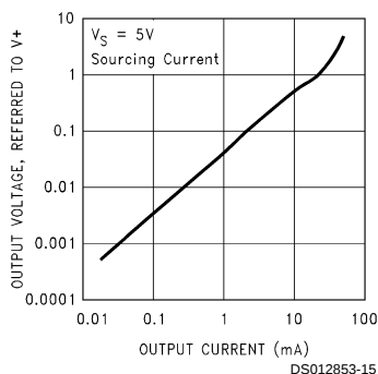
Output Voltage vs Output Current LMC7215
