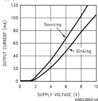
Short Circuit Current vs V_{\text{Supply}}
