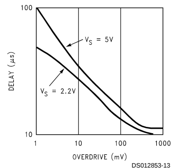
Prop Delay vs Overdrive
