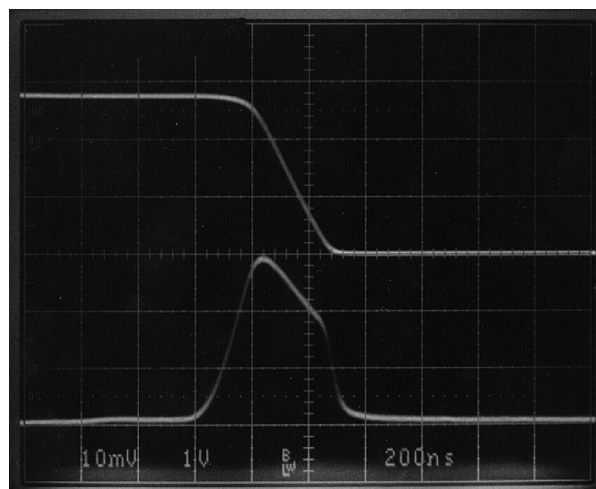
FIGURE 4. R_S = 100\Omega
