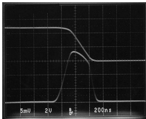
FIGURE 5. R_S = 10\Omega
