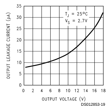
Output Leakage Current vs Output Voltage LMC7225
