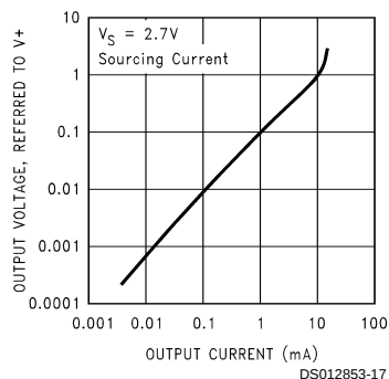
Output Voltage vs Output Current LMC7215
