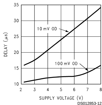
Prop Delay vs V_{\text{Supply}}
