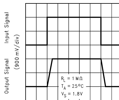
*Large Signal Non-Inverting Response
