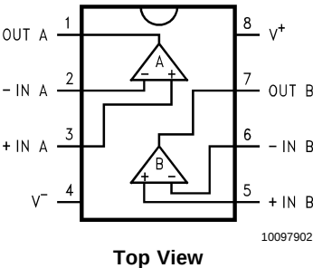
8-Pin MSOP/SOIC
