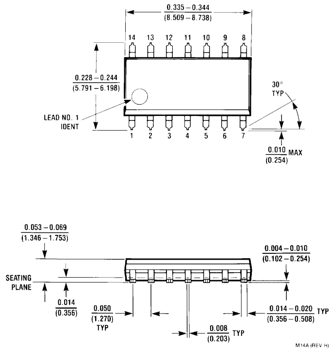
14-Pin SOIC NS Package Number MA14
