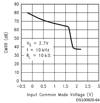
CMRR vs Input Common Mode Voltage
