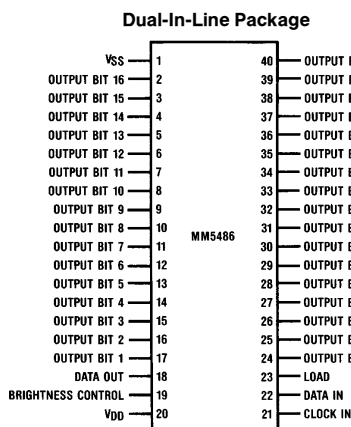
Top View Order Number MM5486N See NS Package Number N40A FIGURE 2
