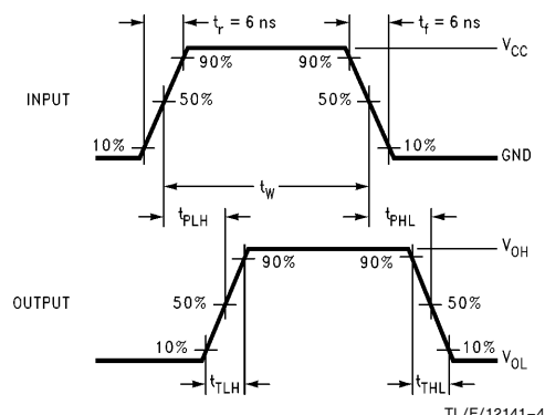
FIGURE 2. AC Waveforms
