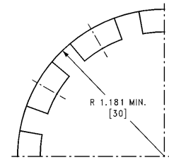
BEND RADIUS NOT TO SCALE TL/F/12167-7
