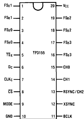
Dual-In-Line Package
