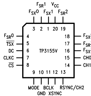
Plastic Chip Carrier (PCC) Package
