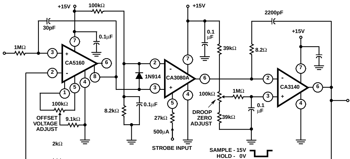
FIGURE 15A. SAMPLE AND HOLD CIRCUIT
