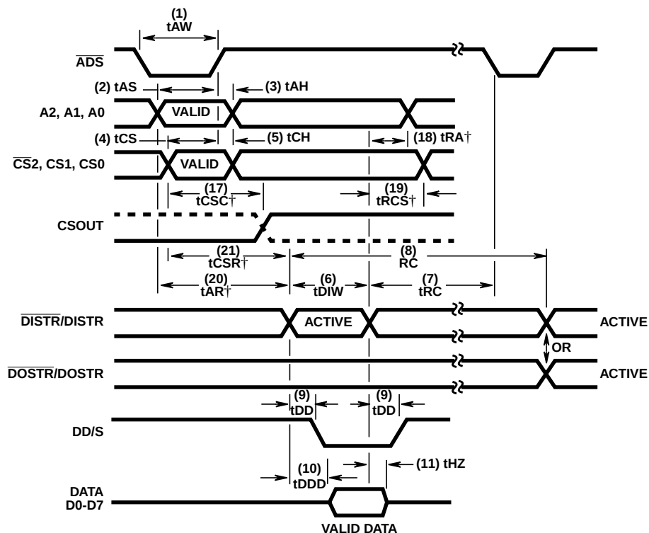
FIGURE 6. WRITE CYCLE
