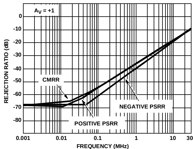
FIGURE 22. REJECTION RATIOS vs FREQUENCY
