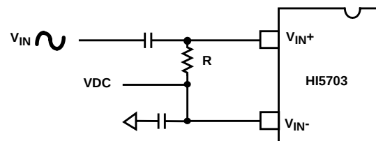
FIGURE 18. AC COUPLED SINGLE ENDED INPUT
