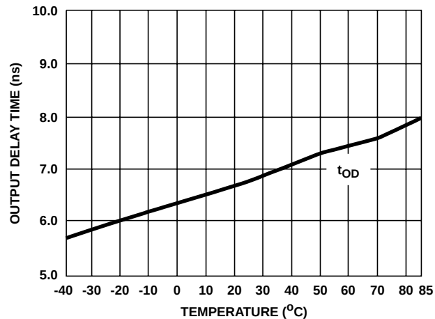
FIGURE 8. OUTPUT DELAY TIME ( T_{OD} ) vs TEMPERATURE
