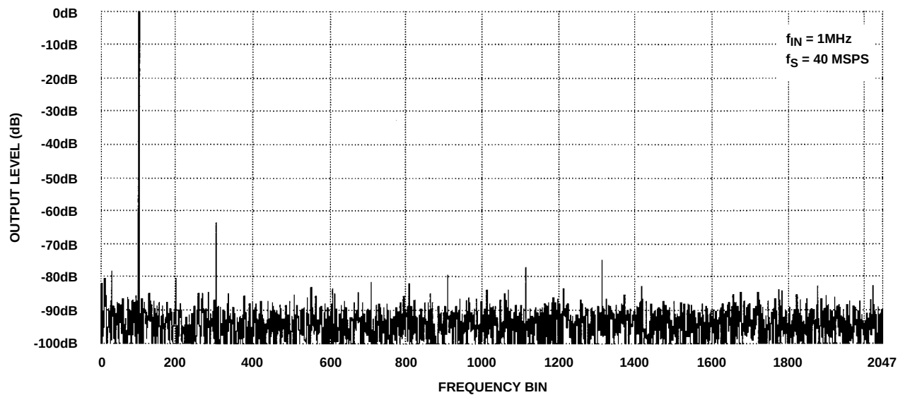
FIGURE 14. 4096 POINT FFT SPECTRAL PLOT
