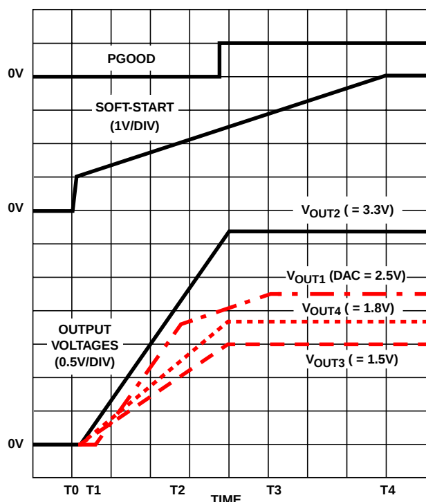
FIGURE 3. SOFT-START INTERVAL
