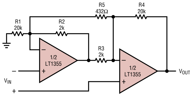
Instrumentation Amplifier
