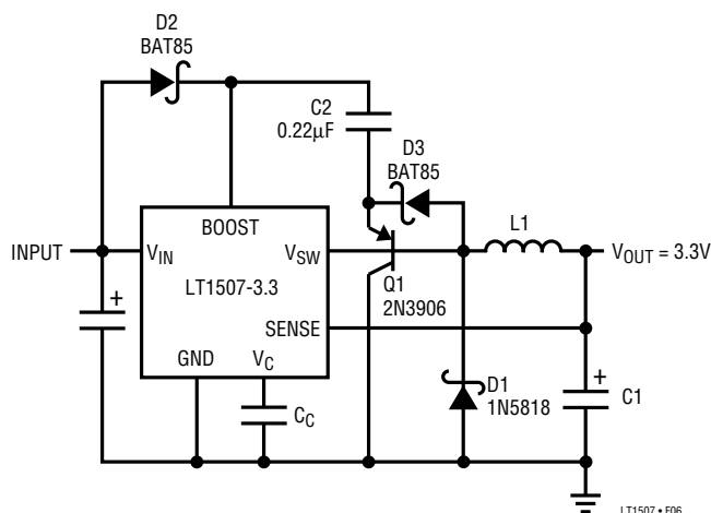
Figure 6. Adding a Small PNP to Reduce Minimum Start-Up Voltage
