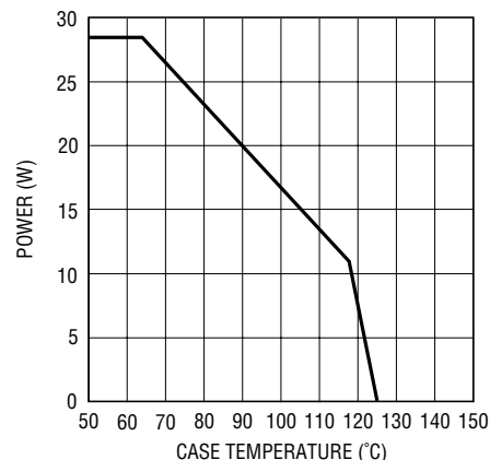
LT1585A Maximum Power Dissipation*
