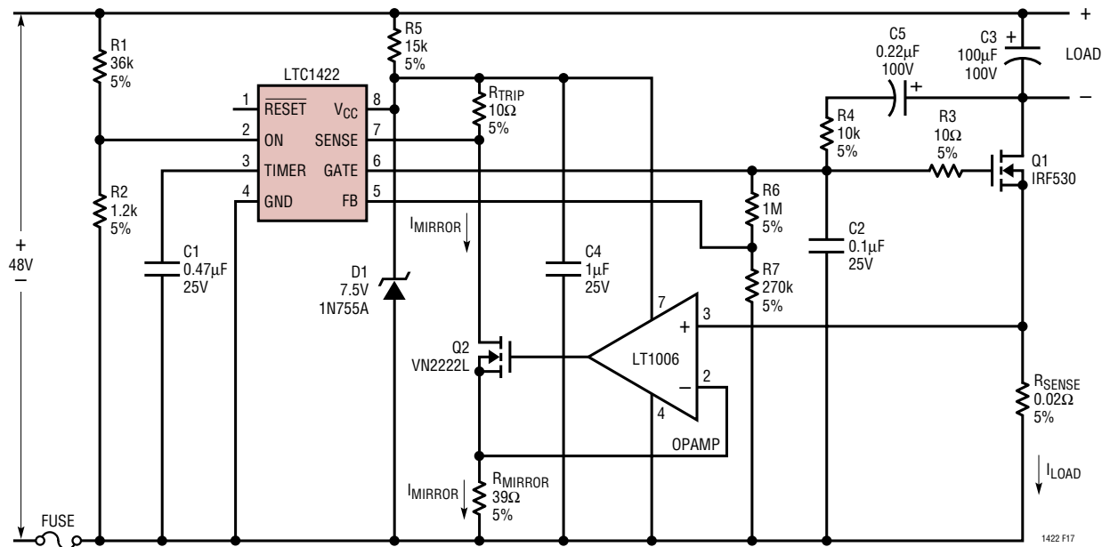
Figure 17. Switching 48V with Current Sensing
