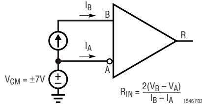
Figure 3. Input Impedance Test Circuit
