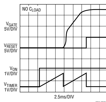
Power-Up Sequence
