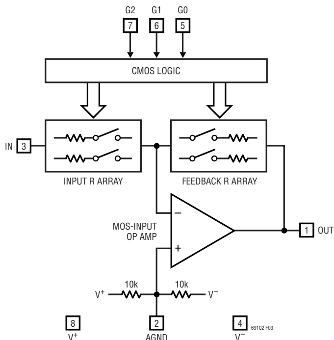
Figure 3. Block Diagram
