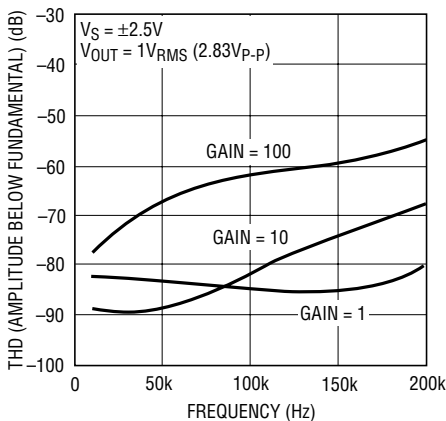
LTC6911-1 Distortion vs Frequency with Light Loading ( R_L = 10k )
