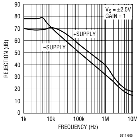
LTC6911-1 Power Supply Rejection vs Frequency
