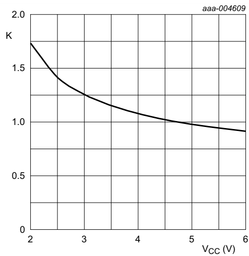
K-factor for 74HC132-Q100
