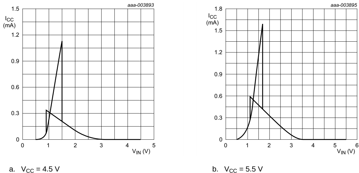
Fig 10. Typical 74HCT132-Q100 transfer characteristics
