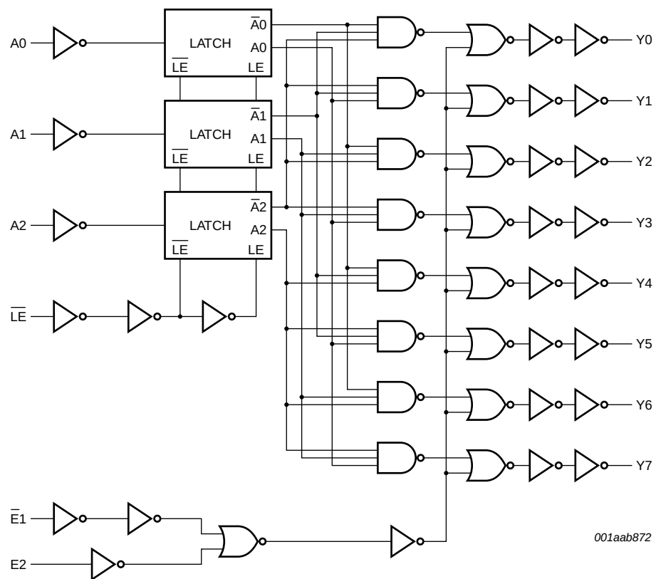
Fig 4. Logic diagram
