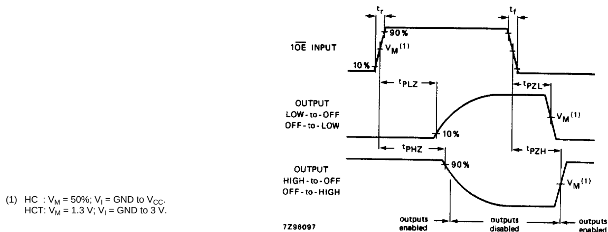
Fig.6 Waveform showing the 3-state enable and disable times for input 1OE .
