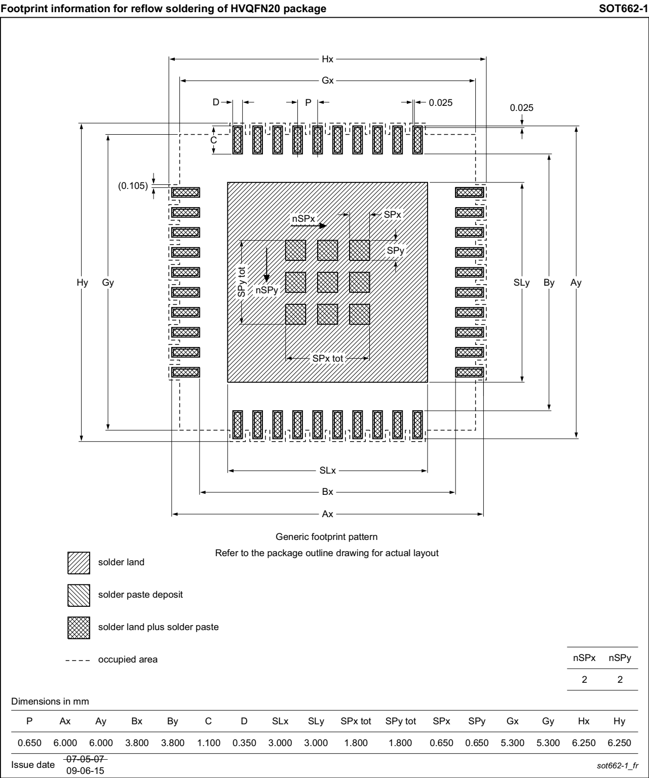
Fig 23. PCB footprint for SOT662-1 (HVQFN20); reflow soldering
