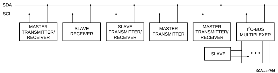
Fig 10. System configuration
