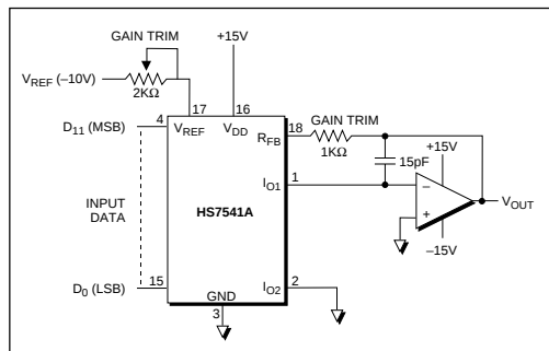
Figure 4. Unipolar Operation
