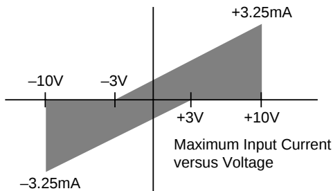
RS423 RECEIVER
