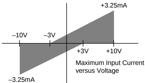
RS422 RECEIVER
