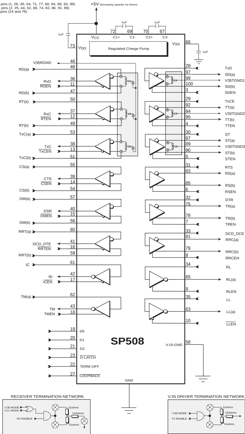
Figure 45. Functional Diagram
