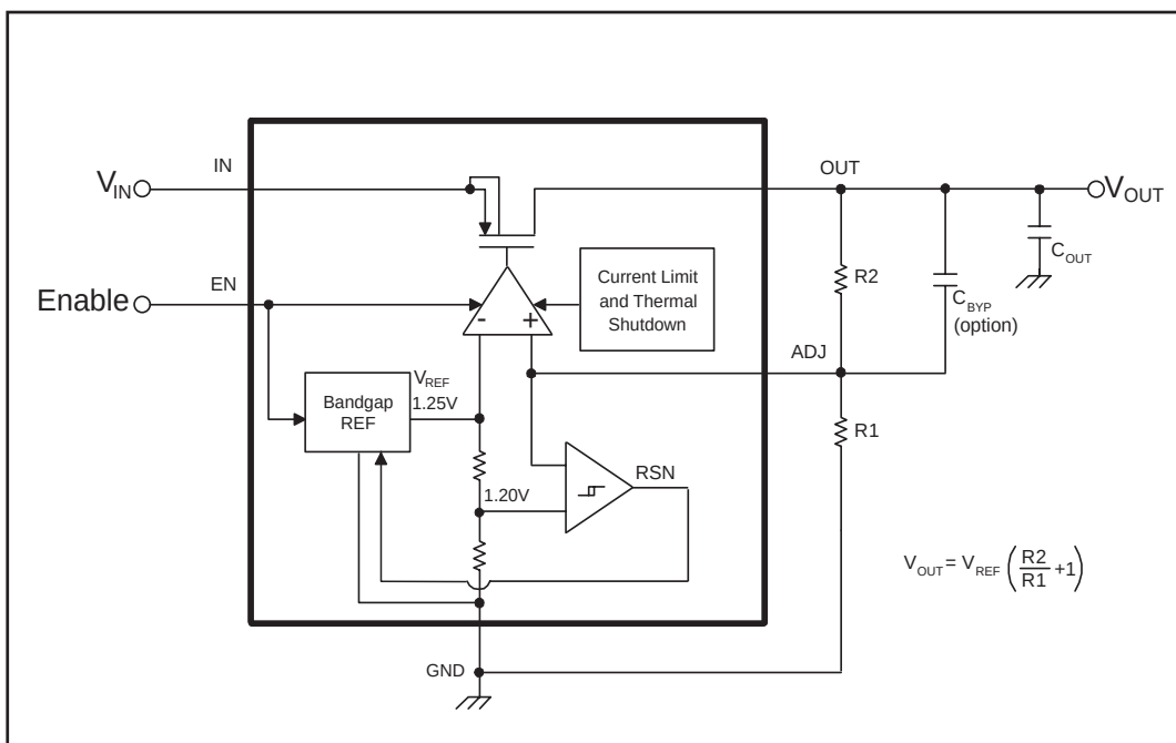
Figure 2. Adjustable Voltage Regulator
