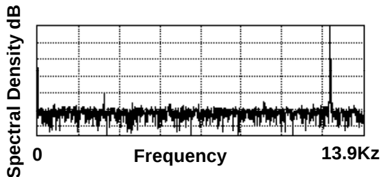
FFT 20 dB/div
