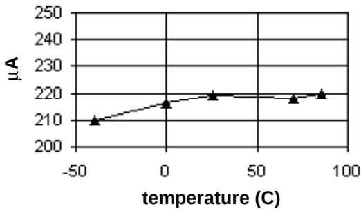
Icc vs. Temperature
