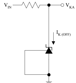
Figure 1c. Test Circuit 3
