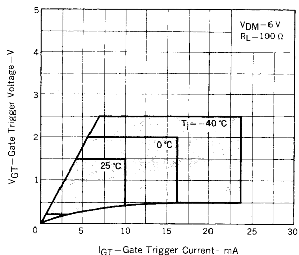
Fig. 4 GATE CHARACTERISTIC
