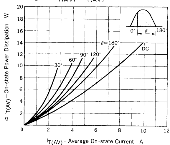
Fig. 10 P_{T(AV)} - I_{T(AV)} CHARACTERISTIC
