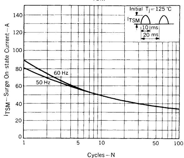
Fig. 2 I_{TSM} RATING
