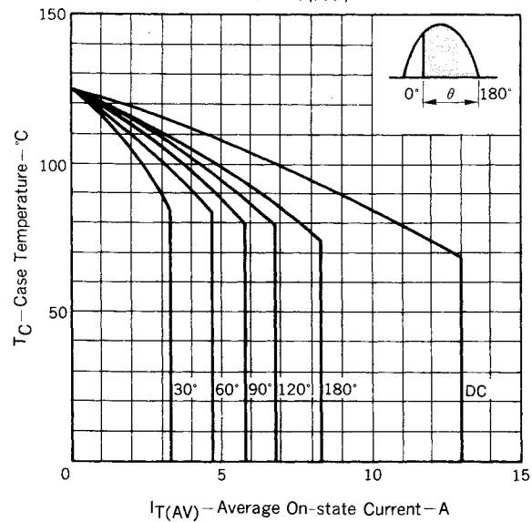
Fig. 11 T_c - I_{T(AV)} RATING
