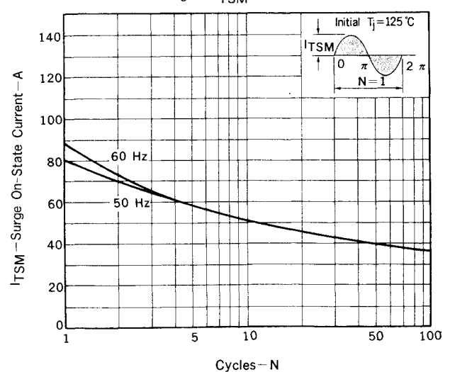
Fig. 2 I_{\text{TSM}} RATING
