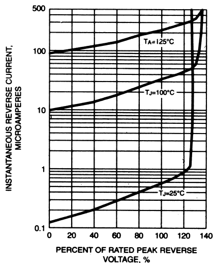
FIG.4-TYPICAL REVERSE CHARACTERISTICS
