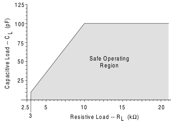
Figure 8. Maximum Loading
