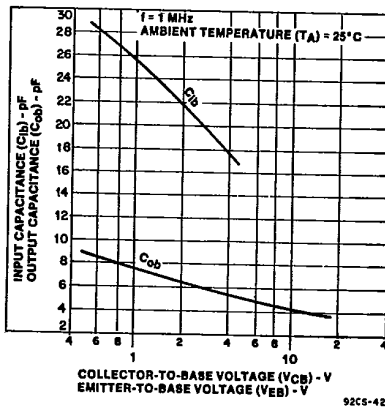
Fig. 7—Typical input and output capacitance characteristics.
