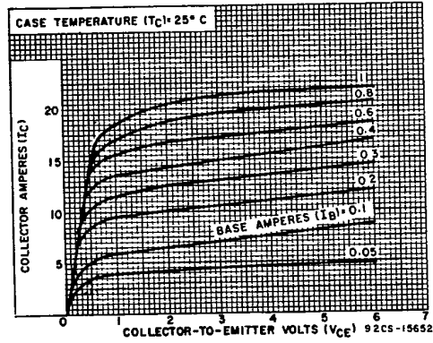
Fig. 5 - Typical output characteristics for types 2N5671 & 2N5672.
