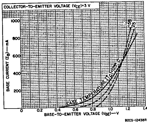
Fig. 4 - Typical input characteristics for types 2N5671 & 2N5672.
