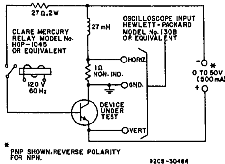
Fig. 11 - Circuit used to measure sustaining voltages V_{CE(sus)} .
