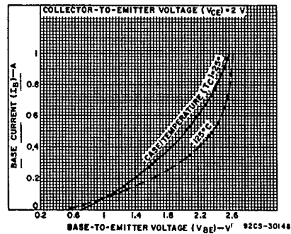
Fig. 5 - Typical input characteristics for MJ15001.
