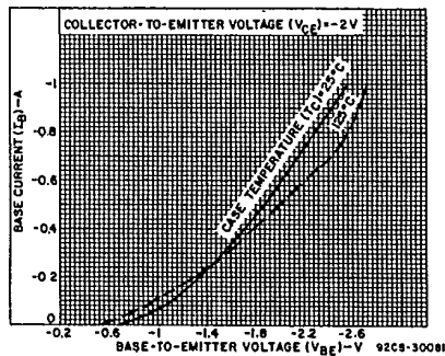
Fig. 6 - Typical input characteristics for MJ15002.
