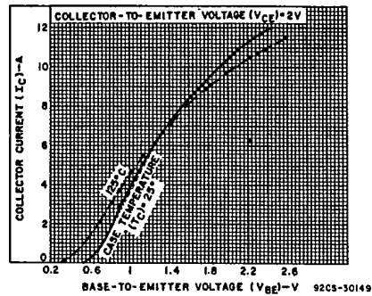
Fig. 7 - Typical transfer characteristics for MJ15001.
