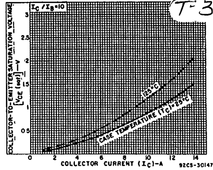
Fig. 9 - Typical saturation voltage characteristics for MJ15001.
