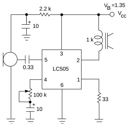
Fig. 12 LC505 Typical Hearing Aid Application
