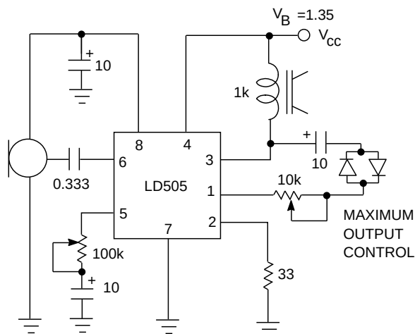
Fig. 13 LD505 Typical Hearing Aid Application
