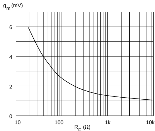
Fig. 11 Transconductance vs Emitter Resistor
