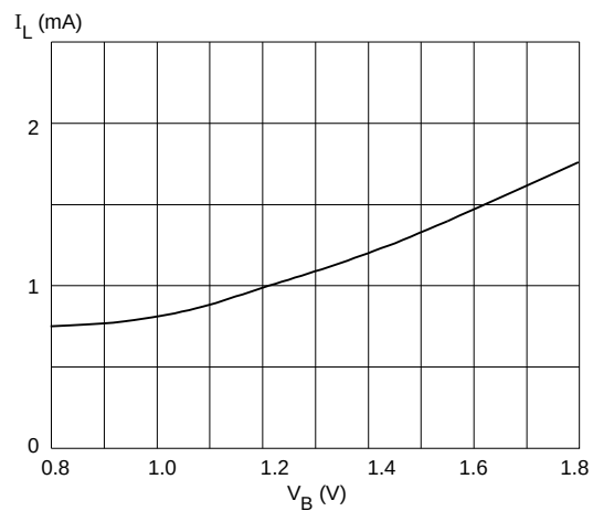
Fig. 6 Load Current vs Supply Voltage
