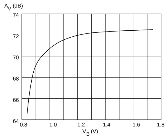
Fig. 7 Absolute Voltage Gain vs Supply Voltage
