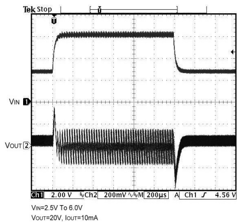
Line Transient
