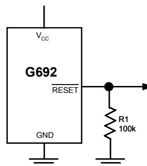
Figure 2. \overline{RESET} Valid to V_{CC} = Ground Circuit
