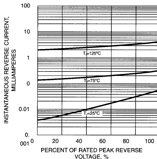
FIG. 4-TYPICAL REVERSE CHARACTERISTICS
