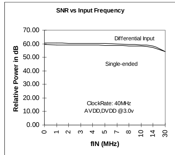
Figure 15. SNR vs Input Frequency, Differential and Single Ended Inputs, V_{DD}=3V
