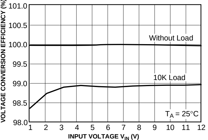
Voltage Conversion
