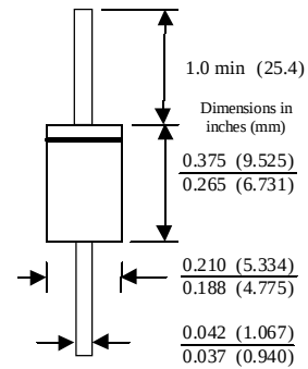
DO-201AE COLOR BAND DENOTES CATHODE
