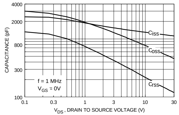
Figure 8. Capacitance Characteristics.
