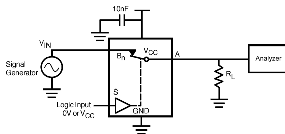
FIGURE 5. Harmonic Distortion
