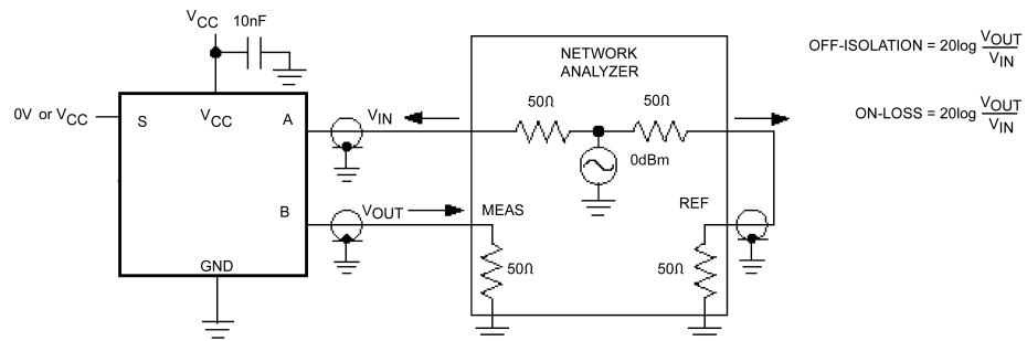
FIGURE 3. OFF Isolation
