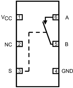
(Top Through View) FSA1157 (Normally Closed)
