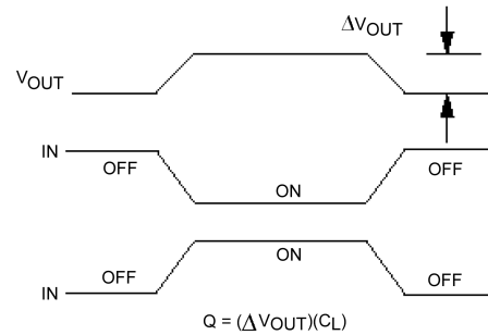
FIGURE 2. Charge Injection
